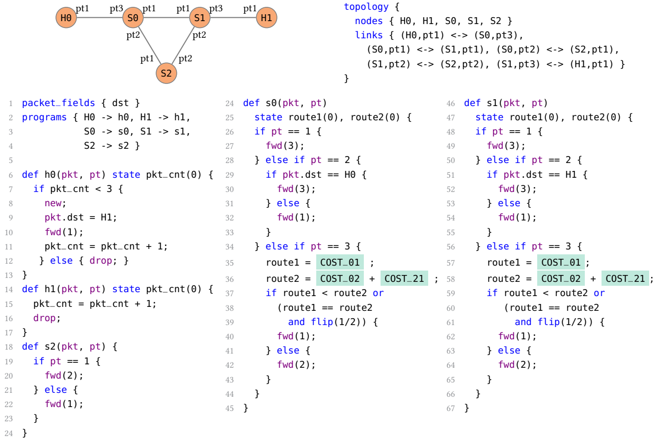
Figure 2. Topology of the network example and its BAYONET representation
