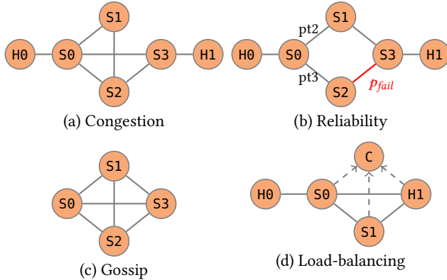
Figure 11. Network topologies used in our benchmarks
