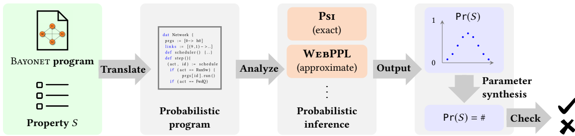
Figure 1. Probabilistic Inference for Networks with BAYONET.
